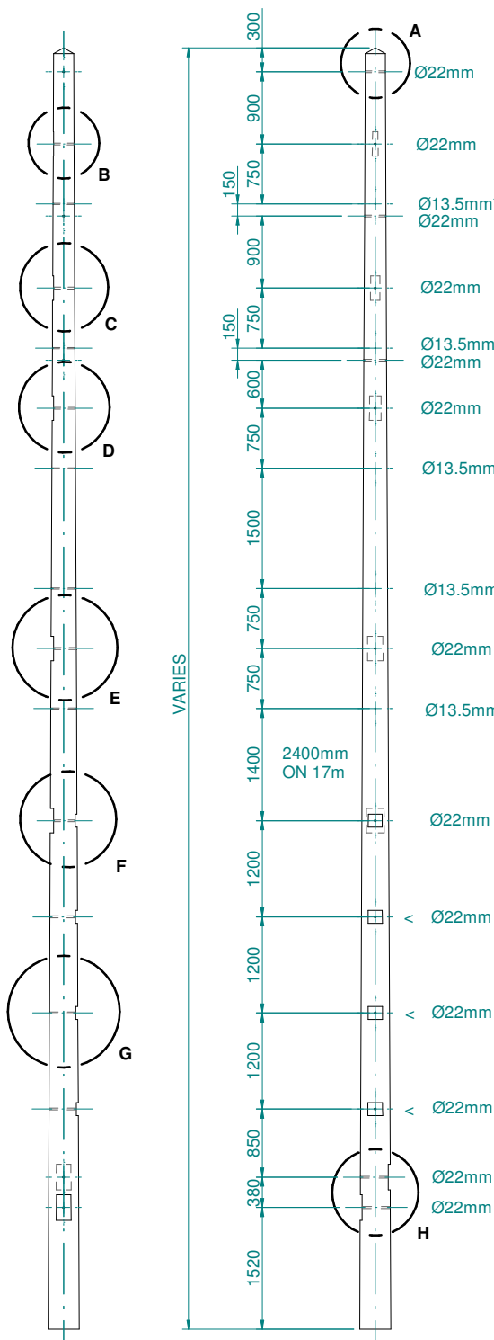
TRANSVERSE ELEVATION
