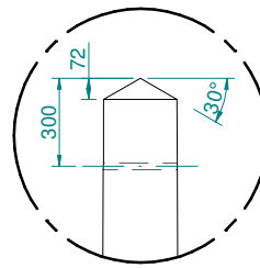
DETAIL A ENLARGED VIEW AT POLE TOP
