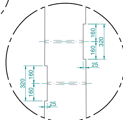
DETAIL H DETAIL ON SCARF FOR FOUNDATION BRACE
