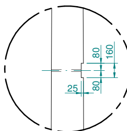
DETAIL G ENLARGED VIEW ON SCARF RELEVANT AT LOCATIONS MARKED "<"
