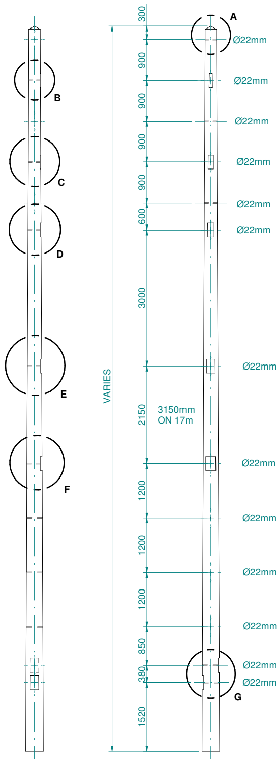
TRANSVERSE ELEVATION
