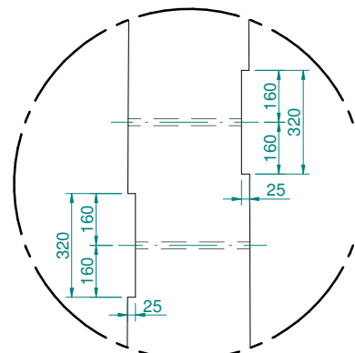
DETAIL G DETAIL ON SCARF FOR FOUNDATION BRACE
